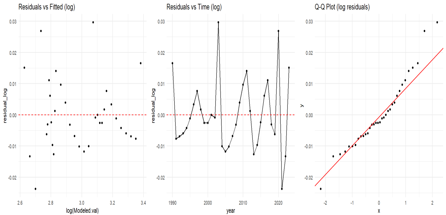
Figure S1. Diagnostic Plots for Assessment of Model Assumptions in the Joinpoint Regression Analysis
